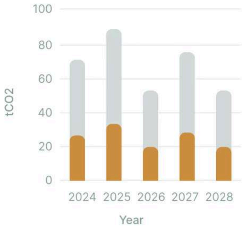
Reduction trajectory
